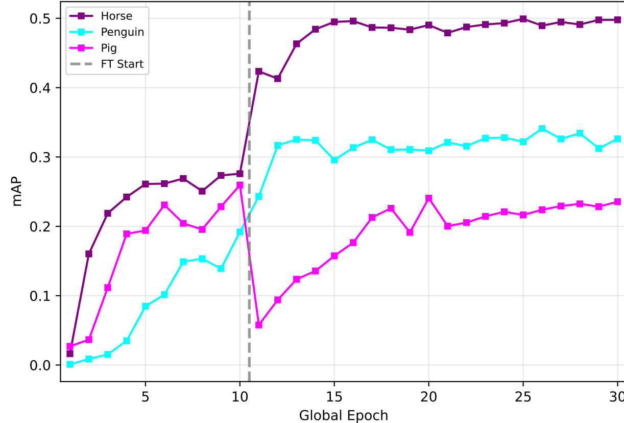
Per-Class mAP
