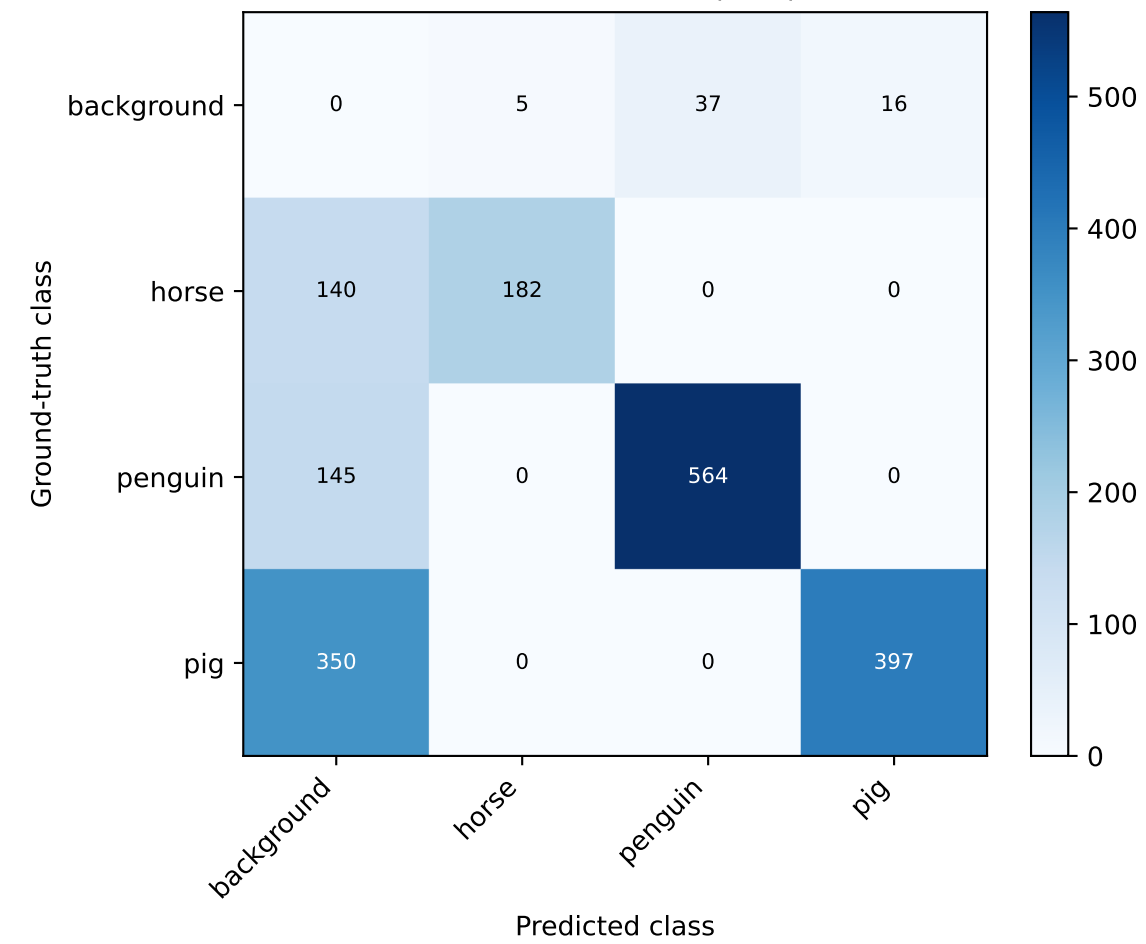
Confusion Matrix (Test)
