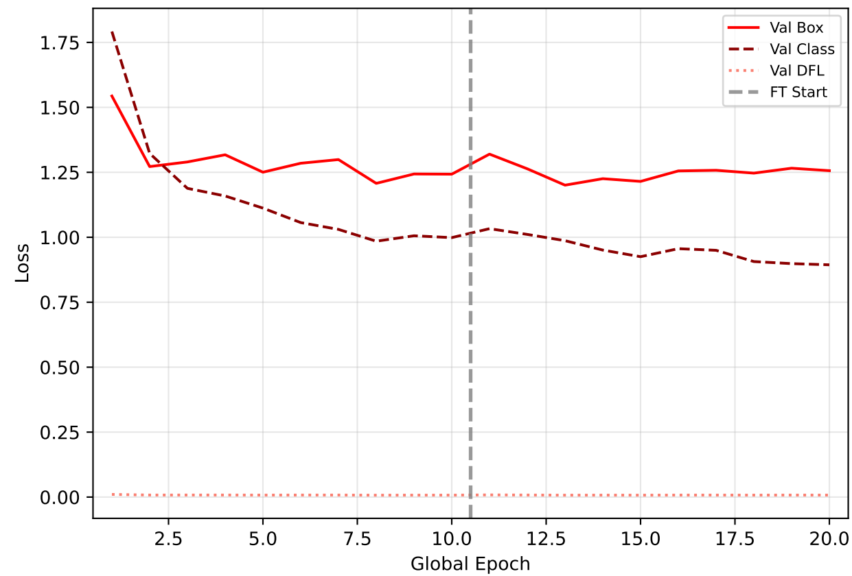
Validation Loss Detail
