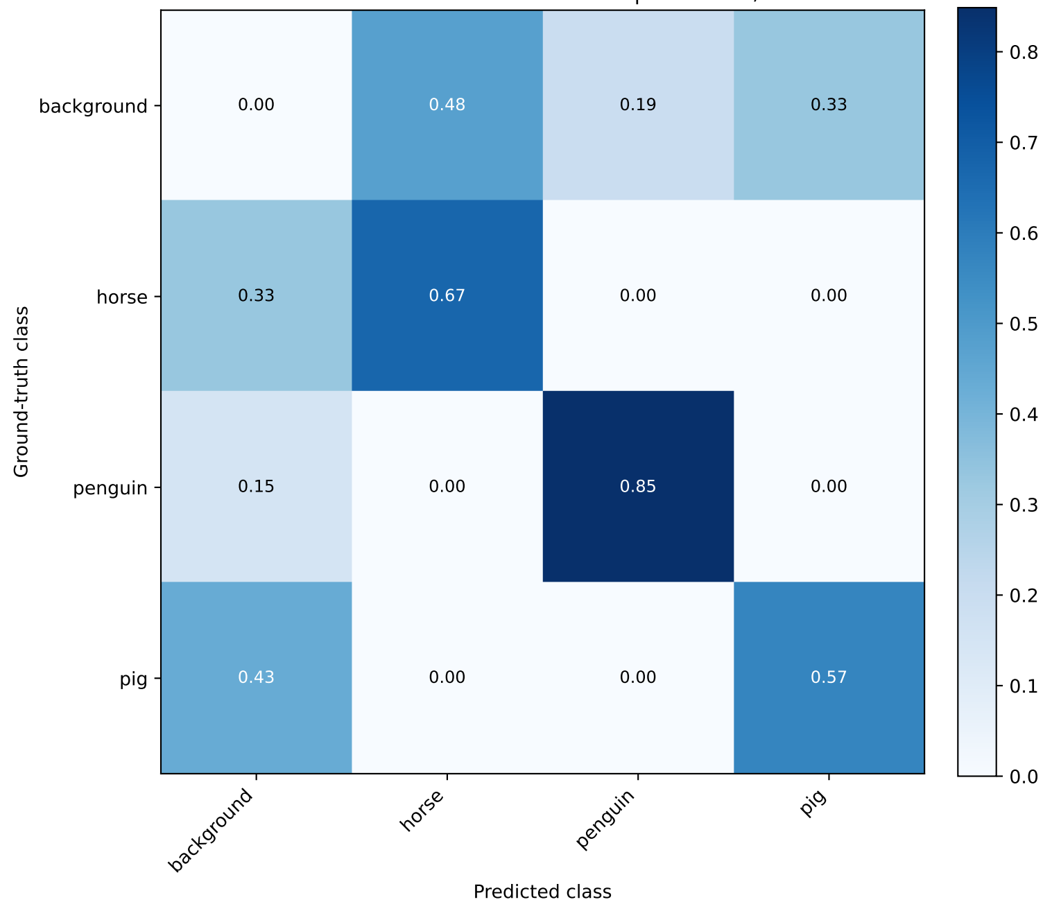
Normalized Detection Confusion Matrix | IoU=0.50, score=0.50
