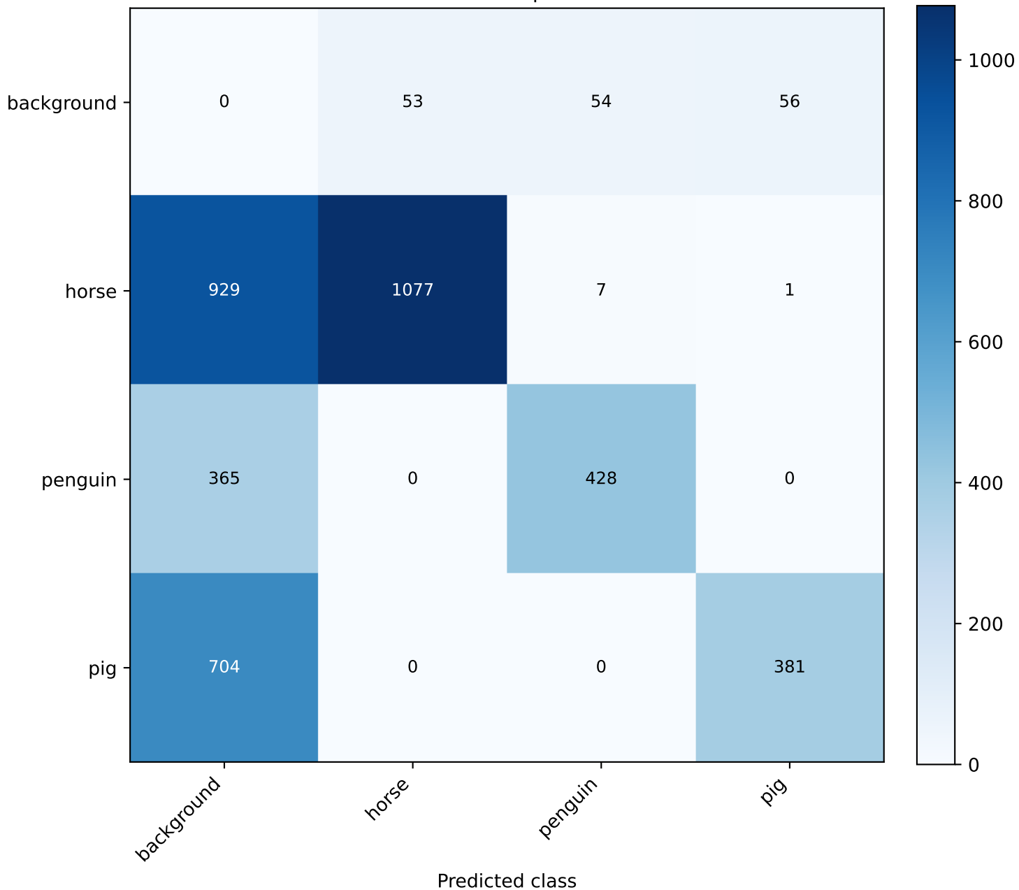
Detection Confusion Matrix | IoU=0.50, score=0.50
