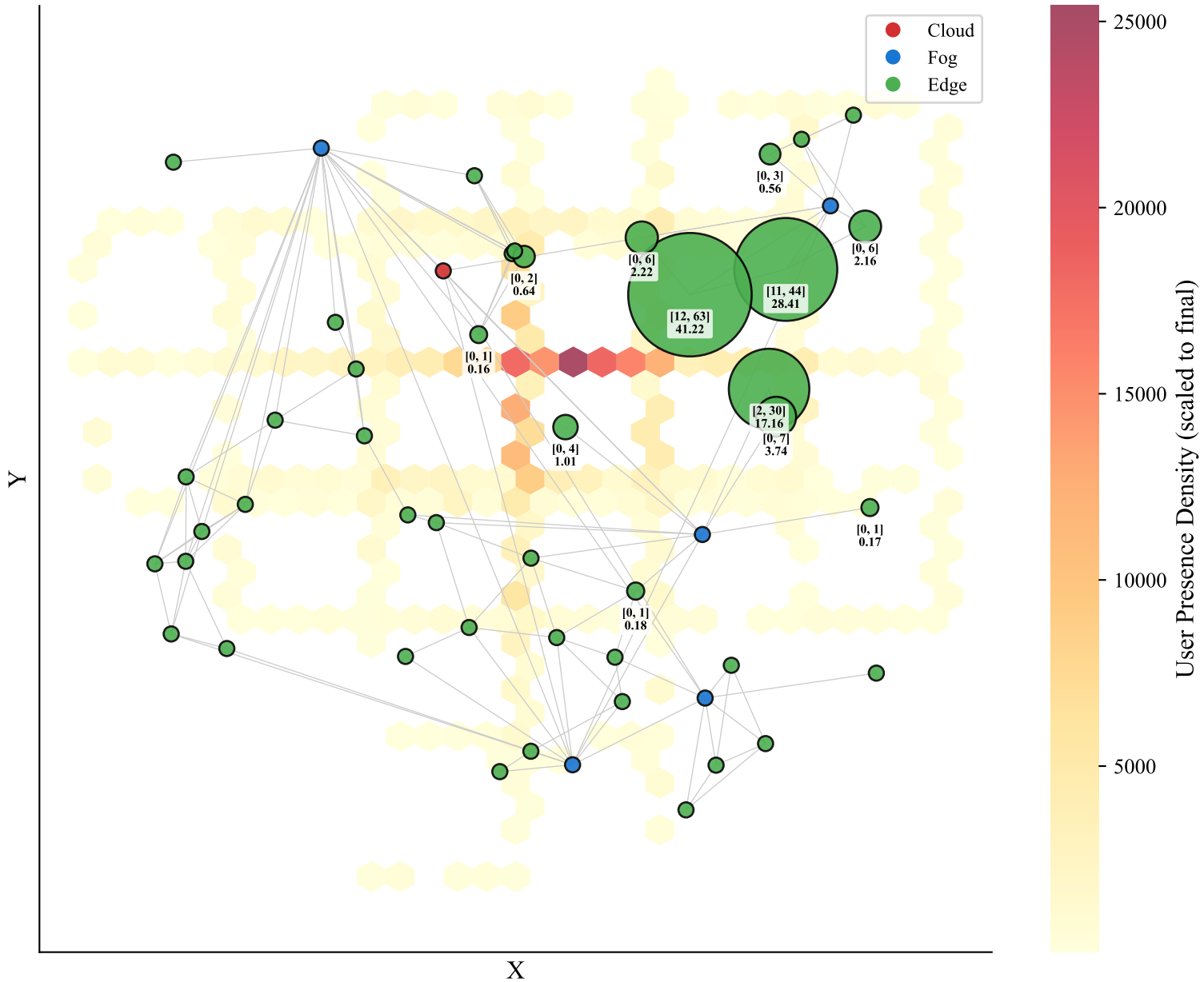
User Mobility Heatmap — 2 Step 4585 — Before Crowd Surge 6
