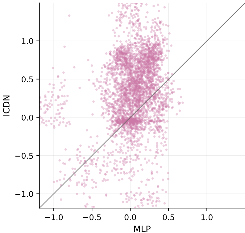
Matched cross-price elasticity — Dominick (beer)
