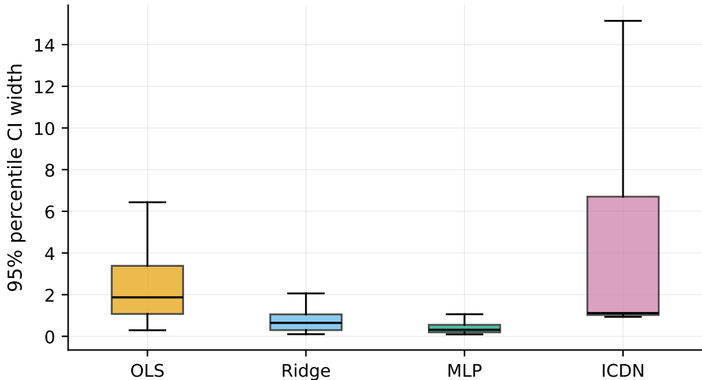
Bootstrap uncertainty (own-price) — 1C (Predict Future Sales)
