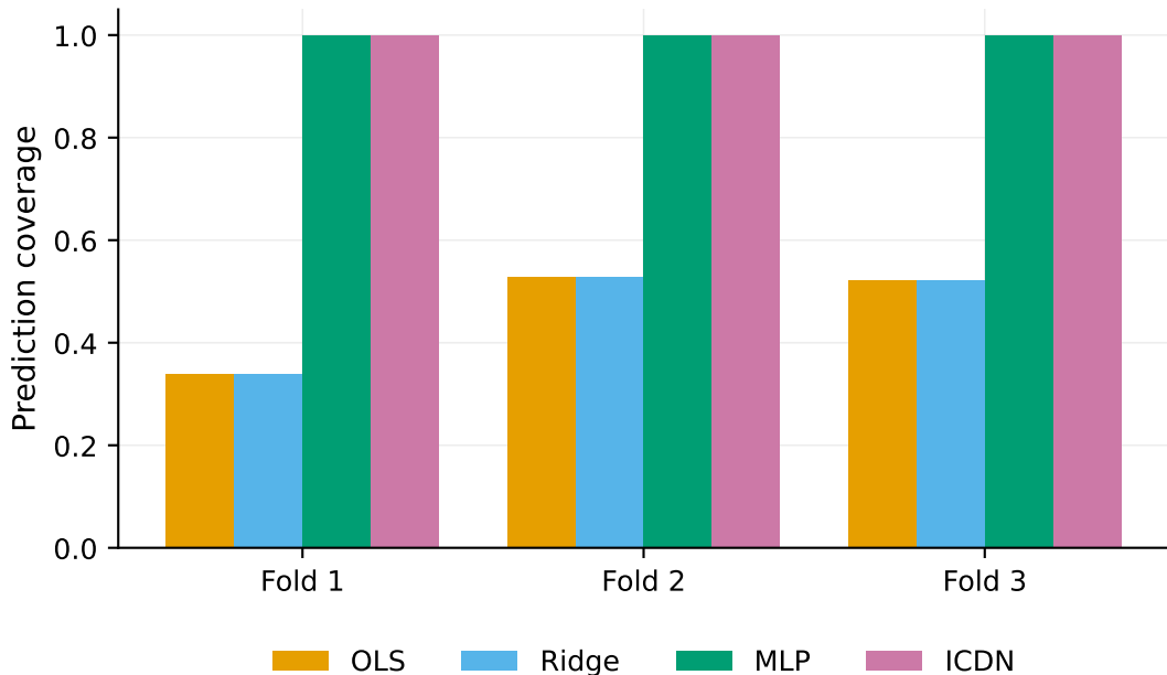
Predicted cells / validation grid — 1C (Predict Future Sales)
