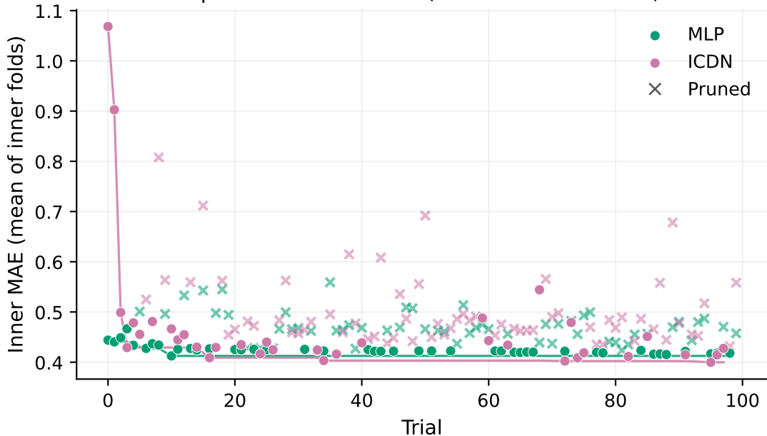
Optuna holdout — 1C (Predict Future Sales)
