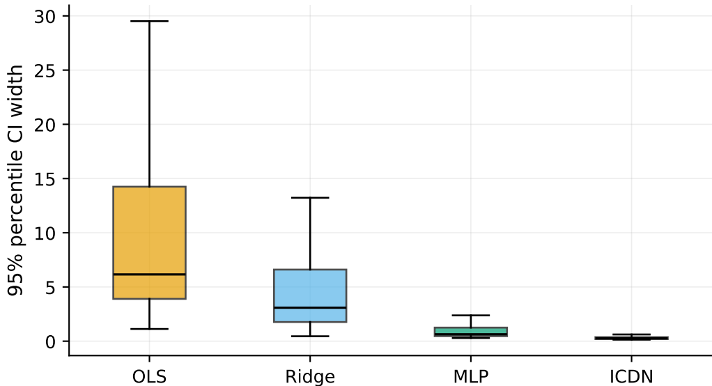
Bootstrap uncertainty (own-price) — Walmart M5 (FOODS_3)
