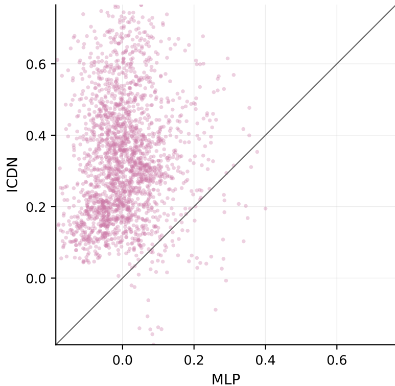
Matched cross-price elasticity — Walmart M5 (FOODS_3)
