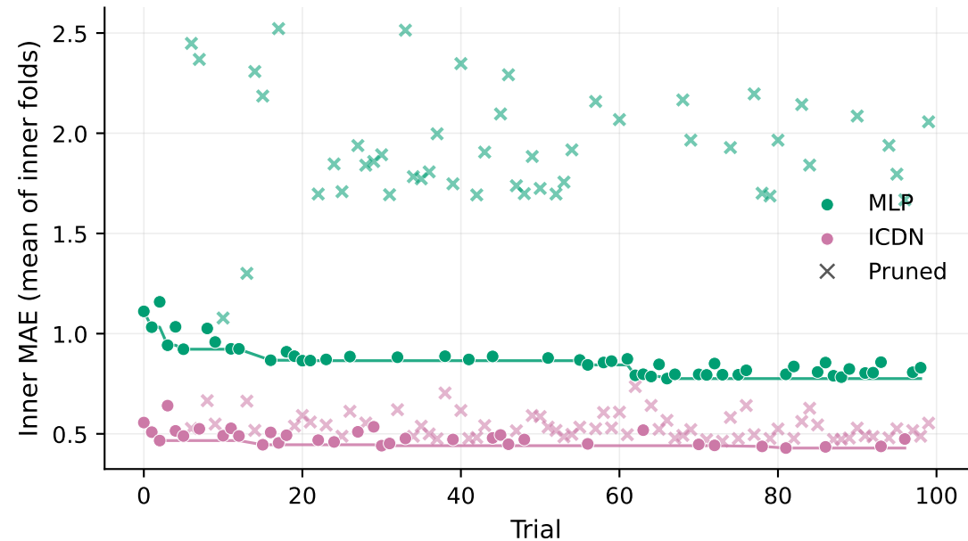
Optuna fold1 — Walmart M5 (FOODS_3)
