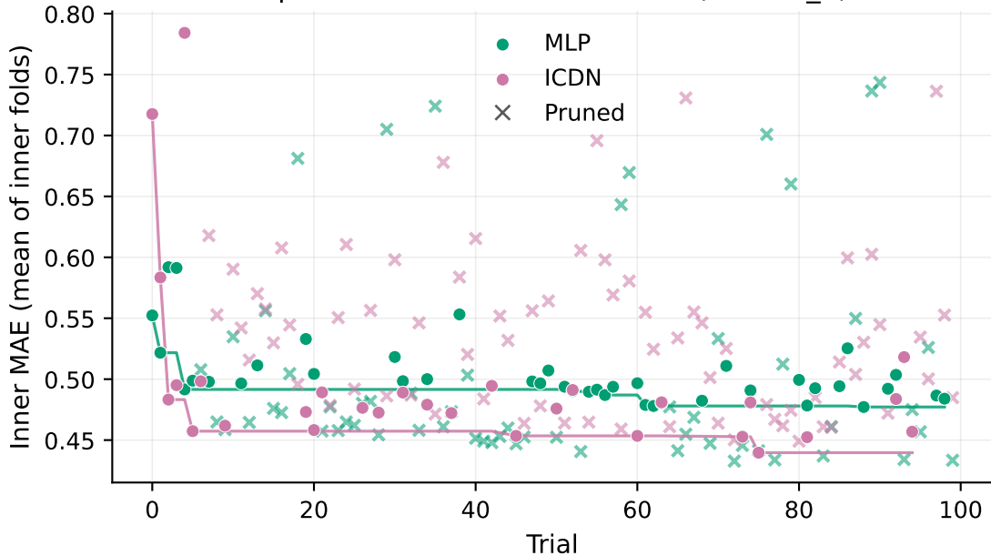
Optuna holdout — Walmart M5 (FOODS_3)
