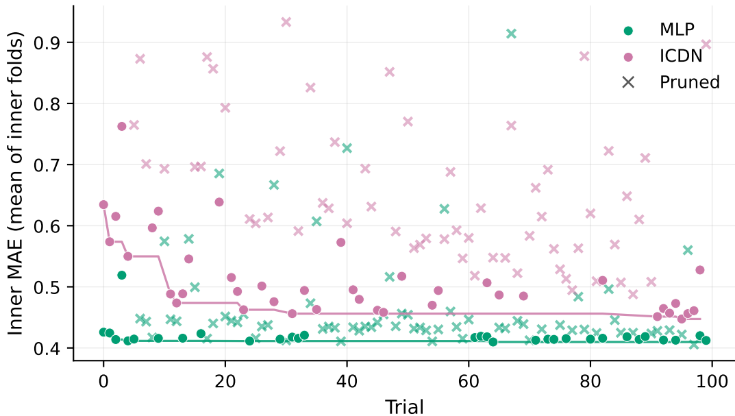
Optuna fold2 — dunnhumby (COLD CEREAL)
