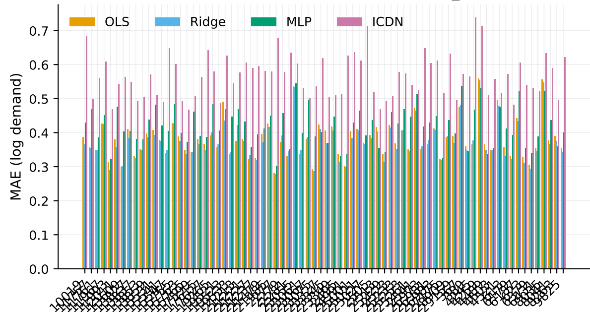
Error by store, fold 1 — Dunnhumby (COLD_CEREAL)
