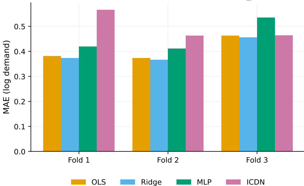
Native prediction error — Dunnhumby (COLD_CEREAL)
