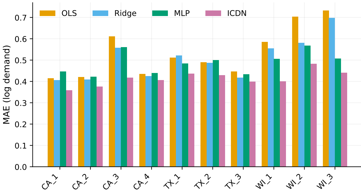
Error by store, fold 1 — Walmart M5 (FOODS_3)
