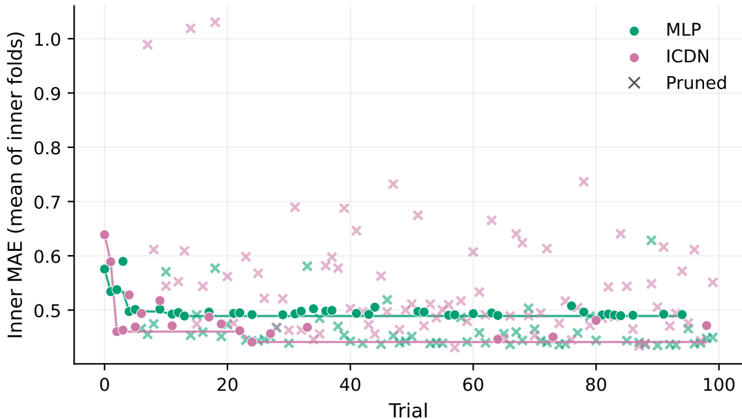
Optuna fold3 — Walmart M5 (FOODS_3)
