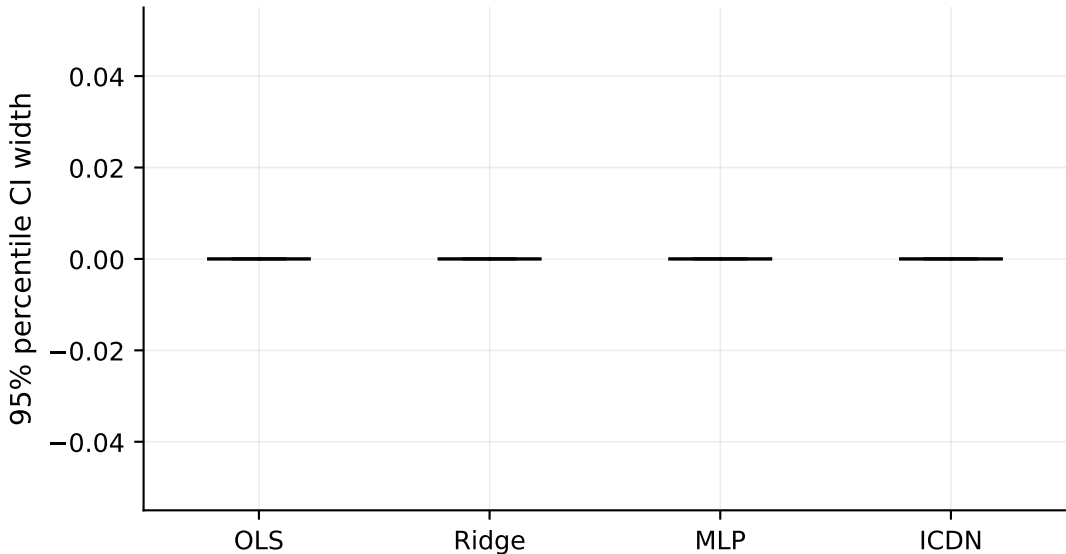
Bootstrap uncertainty (own-price) — dunnhumby (COLD CEREAL)
