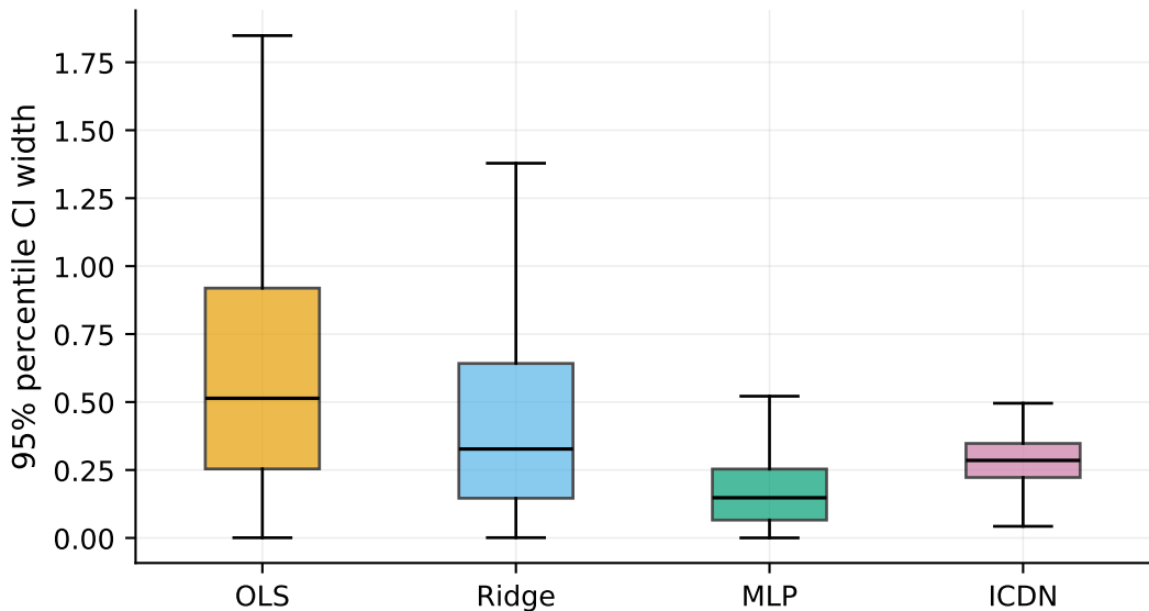
Bootstrap uncertainty (own-price) — Dominick (beer)
