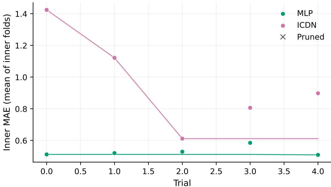
Optuna fold1 — 1C (Predict Future Sales)
