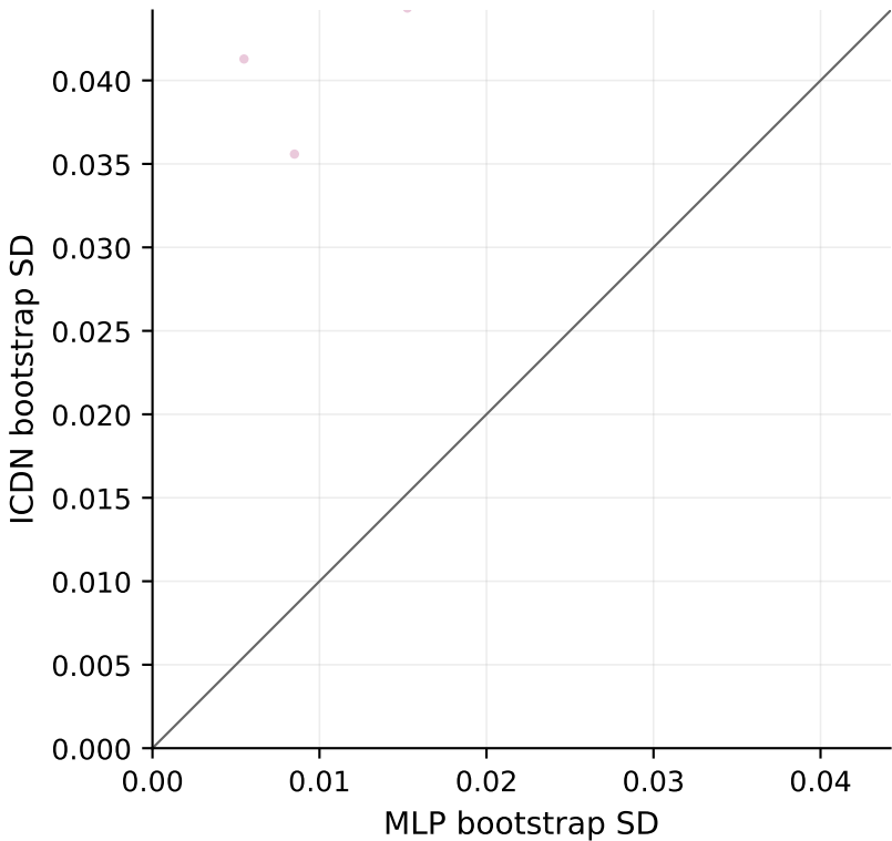
Paired SD (cross-price) — 1C (Predict Future Sales)
