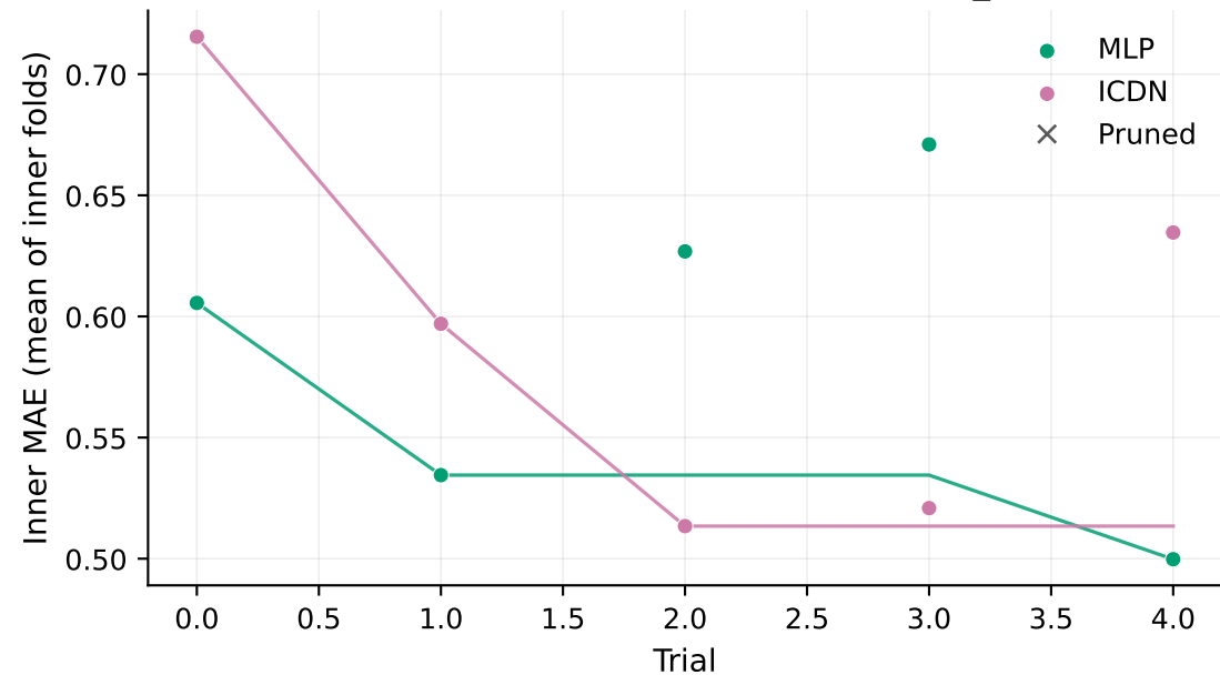
Optuna fold2 — Walmart M5 (FOODS_3)
