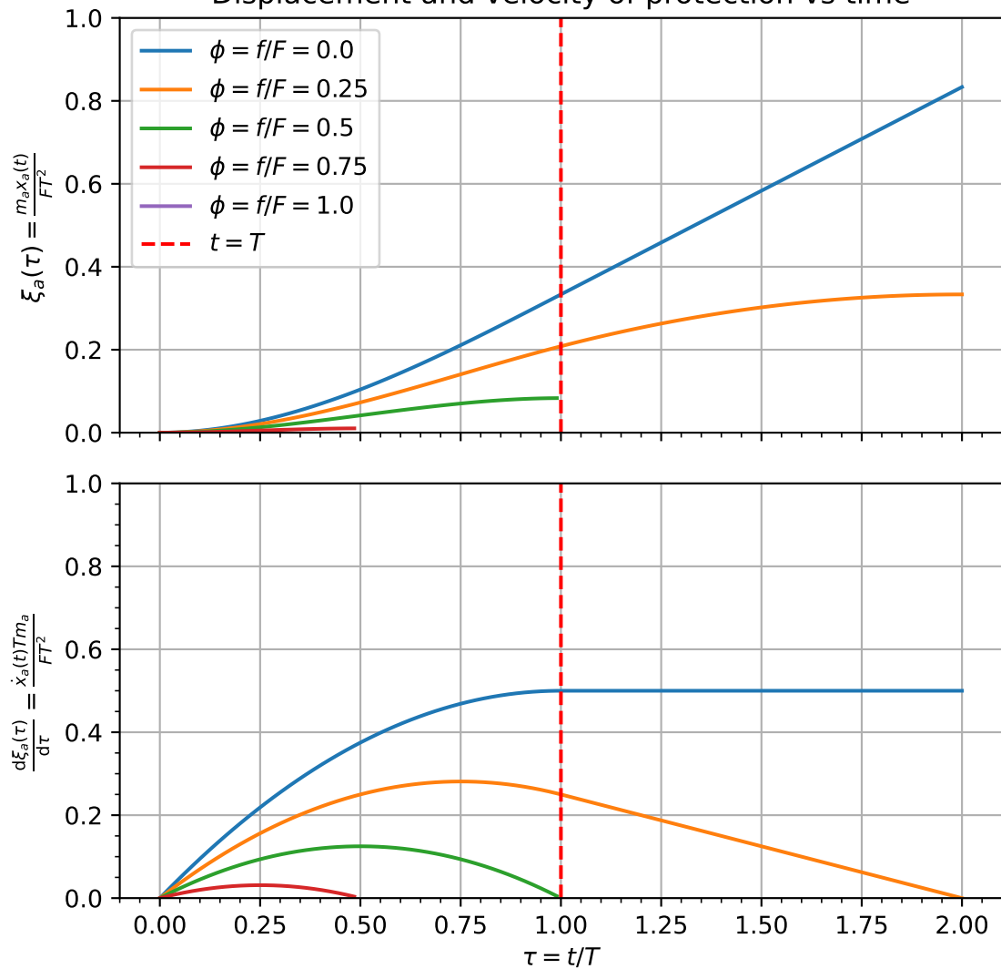
Displacement and velocity of protection vs time
