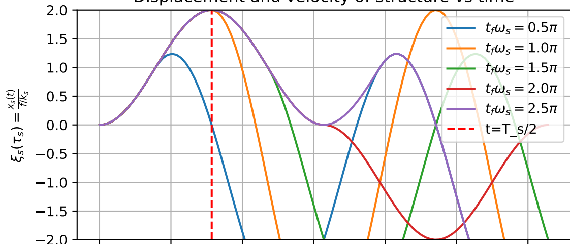
Displacement and velocity of structure vs time
