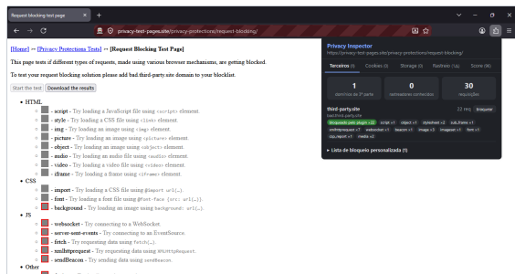
Tracker Blocking (request-blocking) com bad.third-party.site na lista de bloqueio — request-blocking-plugin.png
