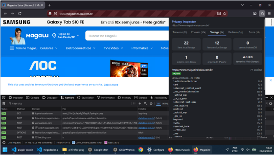
Plugin — aba Storage
