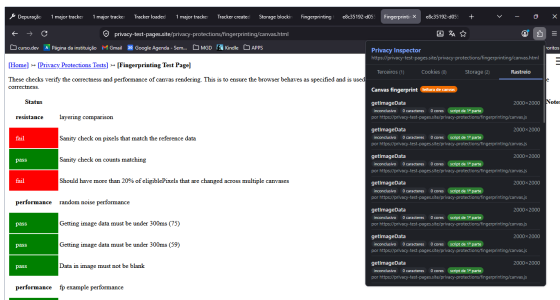
Fingerprinting / canvas.html — fingerprinting-canvas-plugin.png
