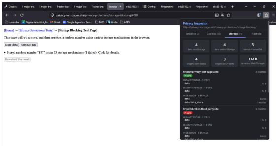
Storage blocking (Store data) — storage-blocking-storage-plugin.png
