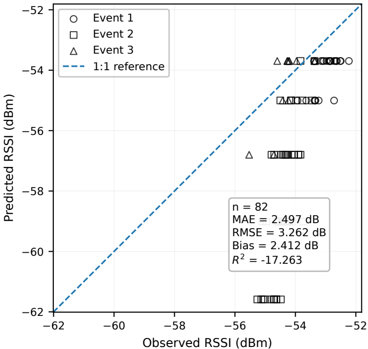
Observed versus predicted RSSI: physical model
