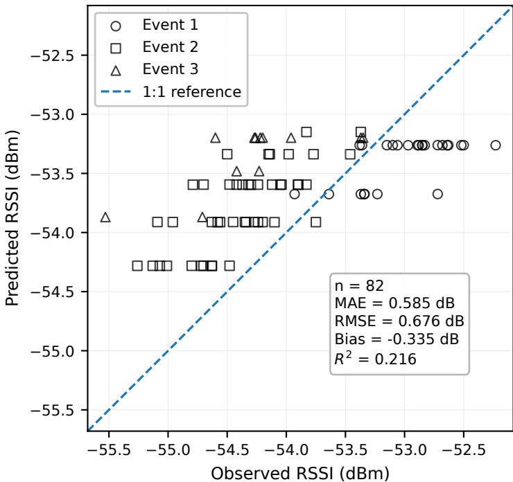
Observed versus predicted RSSI: calibrated model
