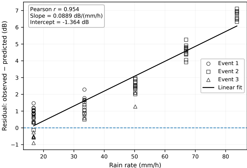
Rain rate versus residual: physical model
