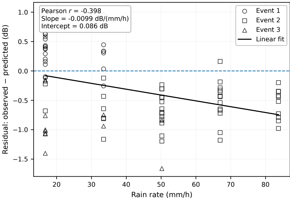
Rain rate versus residual: calibrated model
