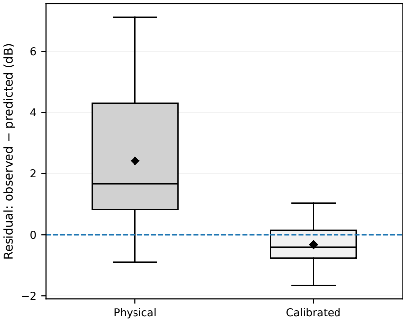
Validation residual distribution
