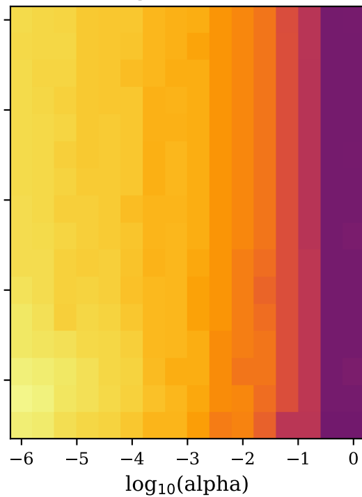
Gauss-Legendre (adaptive)
