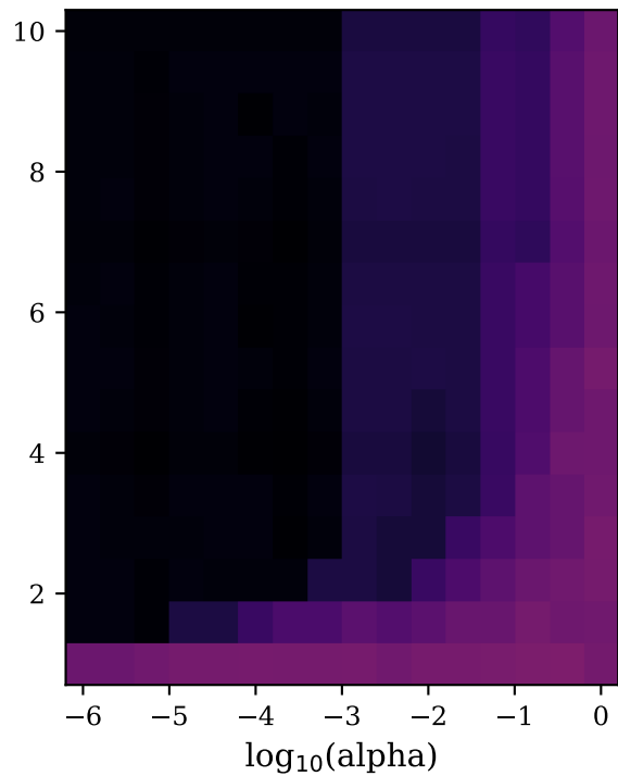
Adaptive series
