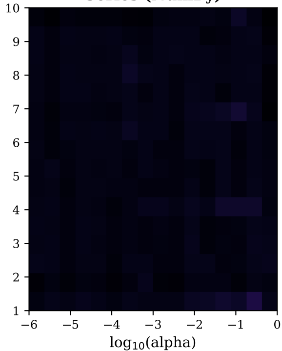
Series (NumPy)
