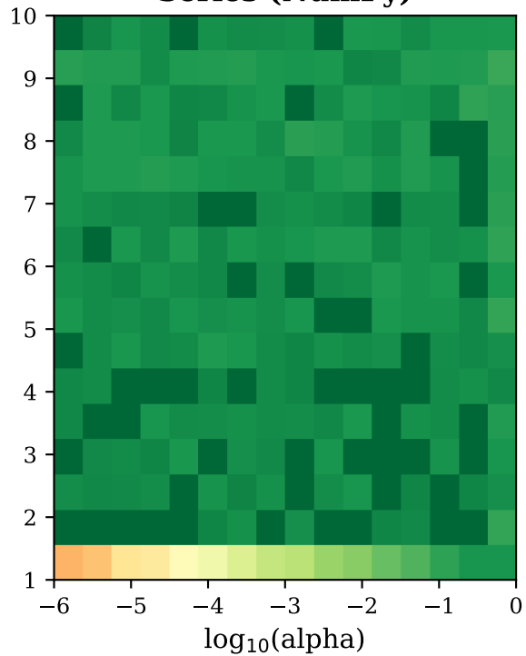
Series (NumPy)
