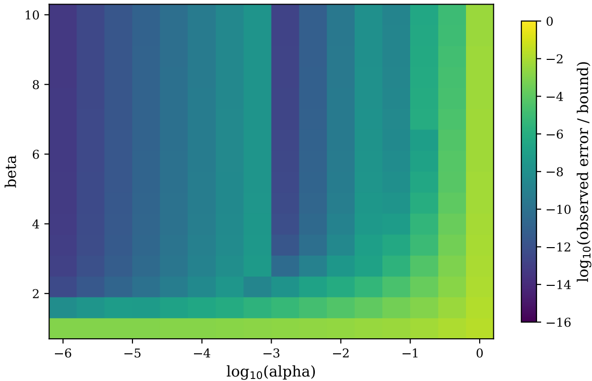
Series Error Relative to Proven Bound
