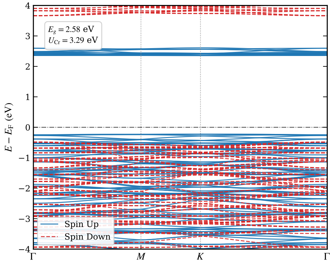
(a) Monolayer \text{CrCl}_3 (+ U_{\text{Cr}} , vdW-D3)
