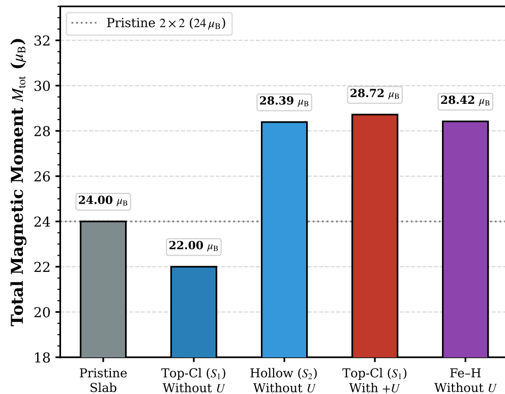
(b) Fe Spin Alignment & Magnetic Coupling
