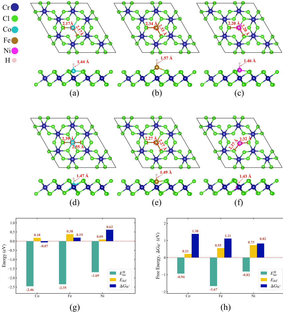
Figure 7: Optimized H-adsorption geometries and energetic decomposition for transition-metal-functionalized monolayer CrCl 3 . (a–c) Surface-adsorbed Co, Fe, and Ni after H adsorption. (d–f) Corresponding embedded configurations. Selected TM–H and local interatomic distances are indicated. (g,h) Atomic-H-referenced interaction energy, E_{\text{int}}^{\text{H}} , deformation energy, E_{\text{def}} , and H adsorption free energy, \Delta G_{\text{H}}^* , for the surface-adsorbed and embedded structures.
