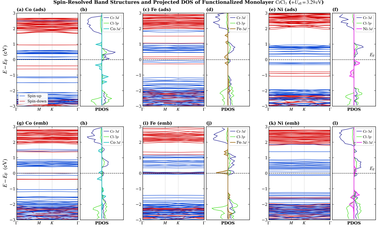
Figure 5: Spin-resolved band structures and projected densities of states of transition-metal-functionalized monolayer \text{CrCl}_3 . Panels (a,b), (c,d), and (e,f) correspond to surface-adsorbed Co, Fe, and Ni, respectively; panels (g,h), (i,j), and (k,l) correspond to the embedded configurations. Blue and red bands denote the spin-up and spin-down channels. The PDOS includes Cr-3d, Cl-3p, and TM-3d contributions, and all energies are referenced to the corresponding Fermi level.
