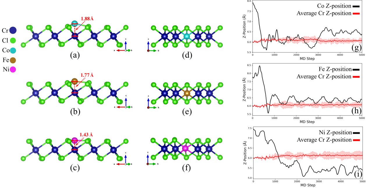
Figure 3: Structural configurations and finite-temperature evolution of Co-, Fe-, and Ni-functionalized monolayer CrCl 3 . (a–c) Optimized surface-adsorbed configurations at the threefold surface hollow site ( S_2 ) considering U_{Cr} = 3.29 eV and vdW corrections. (d–f) Corresponding embedded configurations ( \Delta z_{Cr-TM} \approx 0.0 Å). (g–i) Absolute TM z coordinates during 5 ps AIMD simulations at 300 K. Black curves denote the transition-metal positions; red curves and shaded regions represent the average Cr-plane position and its fluctuations.
