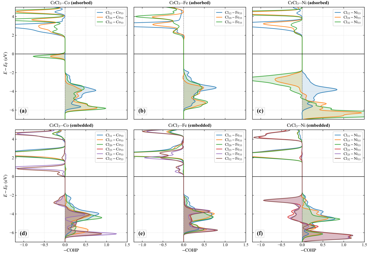
Figure 6: Energy-resolved -COHP curves for individual TM-Cl bonds in transition-metal-functionalized monolayer CrCl_3 . (a-c) Surface-adsorbed Co, Fe, and Ni in threefold coordination. (d-f) Embedded Co, Fe, and Ni in distorted sixfold coordination. The horizontal line marks the Fermi level. Positive -COHP values denote bonding contributions and negative values denote antibonding contributions.
