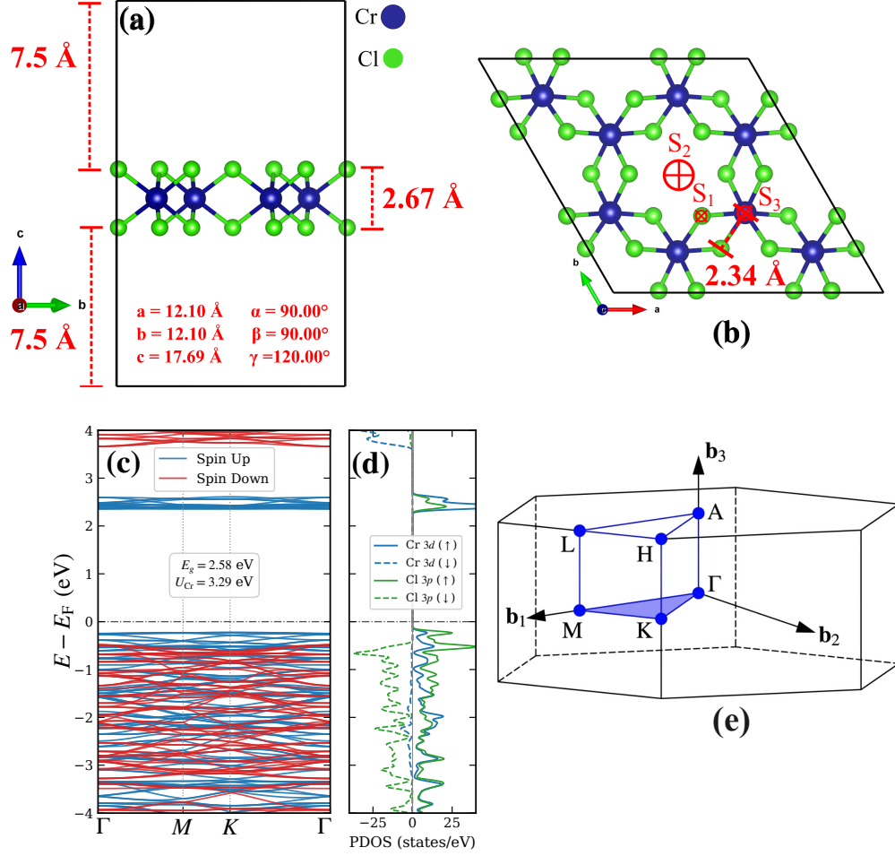
Figure 1: Structural, electronic, and magnetic properties of pristine monolayer \text{CrCl}_3 . (a) Side view of the optimized monolayer in the periodic simulation cell, including the lattice parameters, monolayer thickness, and vacuum spacing. (b) Top view showing a representative Cr-Cl bond length and the hollow site considered for transition-metal functionalization. (c) Spin-resolved band structure along \Gamma -M-K- \Gamma , with the Fermi level set to 0 eV. (d) Projected density of states of the Cr-3d and Cl-3p orbitals. (e) First Brillouin zone and the high-symmetry path used for the band-structure calculations.
