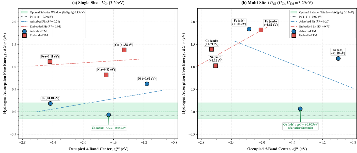
Figure 8: Occupied d -band center, \epsilon_d^{\text{occ}} , versus hydrogen adsorption free energy, \Delta G_{H^*} , for surface-adsorbed and embedded Co, Fe, and Ni centers in monolayer \text{CrCl}_3 across two systematic Hubbard U tiers: (a) single-site +U_{\text{Cr}} ( U_{\text{Cr}} = 3.29 eV) and (b) multi-site +U_{\text{all}} ( U_{\text{Cr}} = U_{\text{TM}} = 3.29 eV; consolidated in Table 1) with explicit vibrational zero-point and entropic corrections. Linear fits are included only as visual guides because each coordination family contains three data points. Shaded green bands denote the optimal Sabatier catalytic window ( |\Delta G_{H^*}| \leq 0.15 eV) with the Pt(111) benchmark ( -0.09 eV) indicated by dotted horizontal lines.
