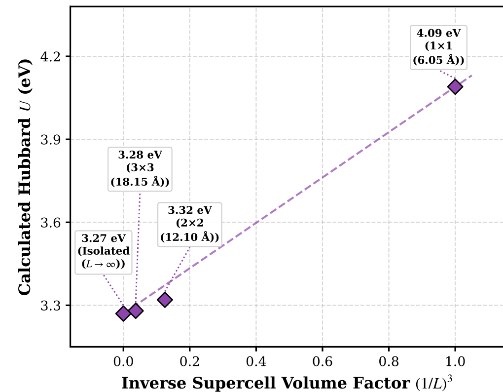
(c) Supercell Finite-Size Scaling & Periodic Image Screening
