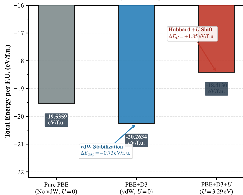
(c) Ground-State Energetics &amp; Dispersion Contribution
