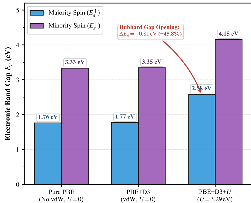
(a) Electronic Band Gap Opening via On-Site Coulomb U
