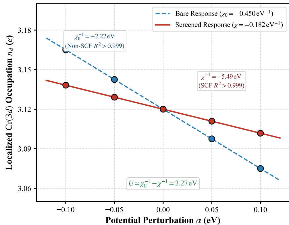
(a) Cococcioni Linear Response on \text{CrCl}_3 ( 2 \times 2 )
