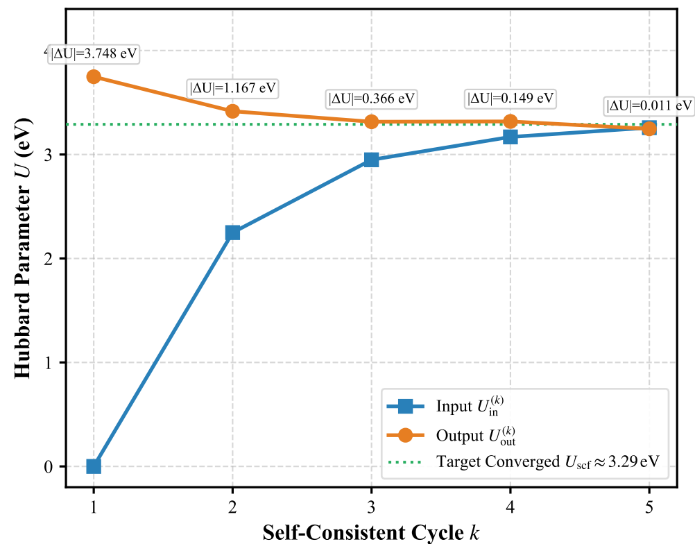
(b) Kulik–Marzari Self-Consistent Feedback Convergence
