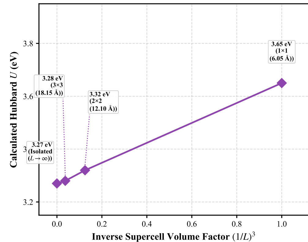
(c) Supercell Finite-Size Scaling & Inter-Image Intersite Screening
