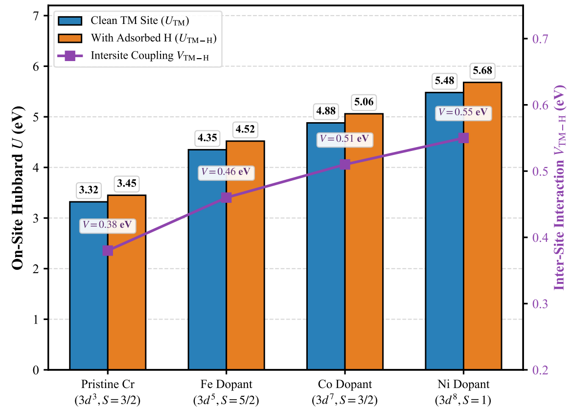
(b) 3d Radial Contraction & Adsorption-Induced Localization
