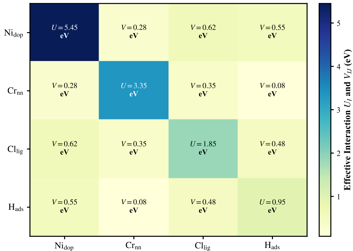
(a) Multi-Site DFT+ U + V Response Tensor (Ni@CrCl 3 + H)
