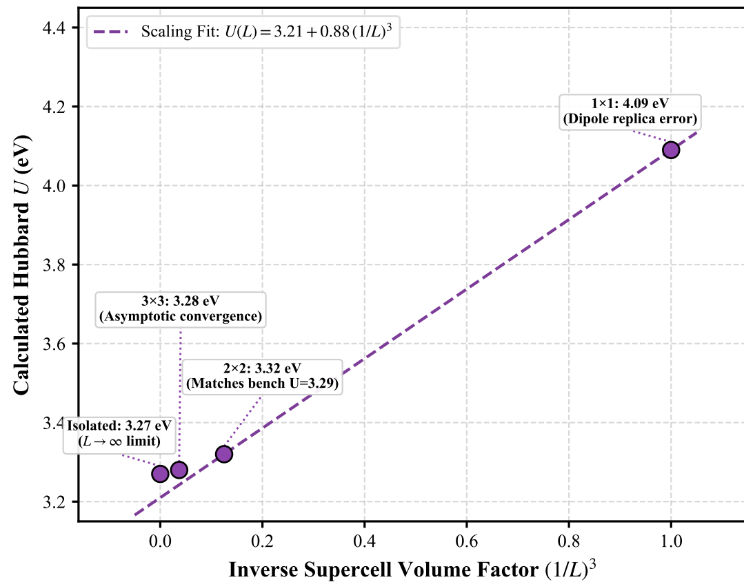
(c) Supercell Scaling & 1/L^3 Inter-Image Polarization Decay
