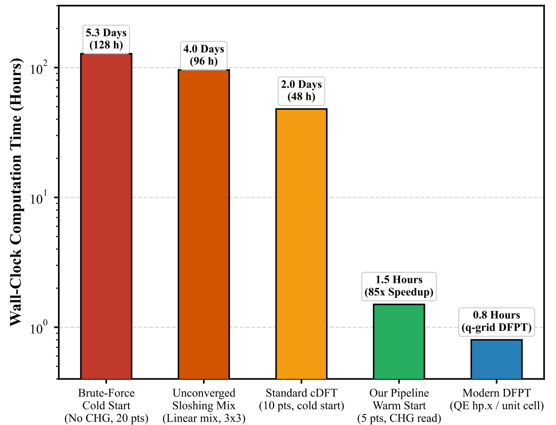
(d) Complexity Audit: Why Brute-Force cDFT Takes 5 Days vs Our Optimized Workflow
