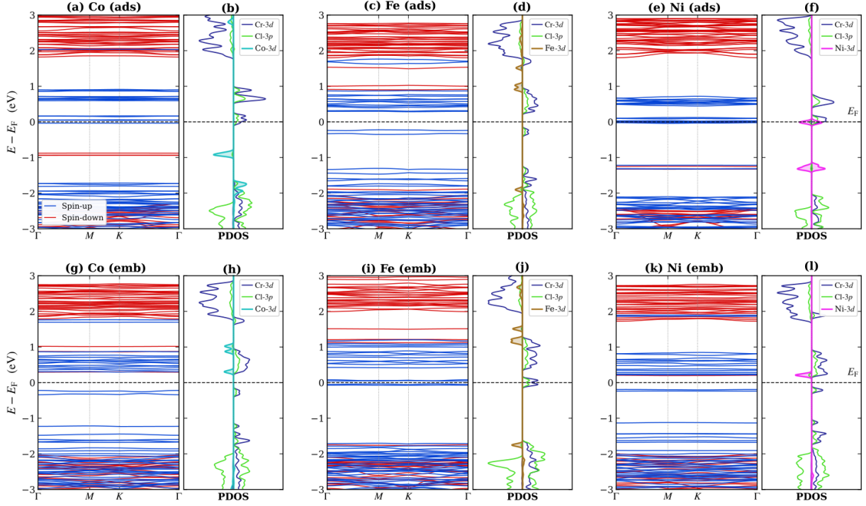
Figure 5: Spin-resolved band structures and projected densities of states of transition-metal-functionalized monolayer \text{CrCl}_3 . Panels (a,b), (c,d), and (e,f) correspond to surface-adsorbed Co, Fe, and Ni, respectively; panels (g,h), (i,j), and (k,l) correspond to the embedded configurations. Blue and red bands denote the spin-up and spin-down channels. The PDOS includes Cr-3d, Cl-3p, and TM-3d contributions, and all energies are referenced to the corresponding Fermi level.
