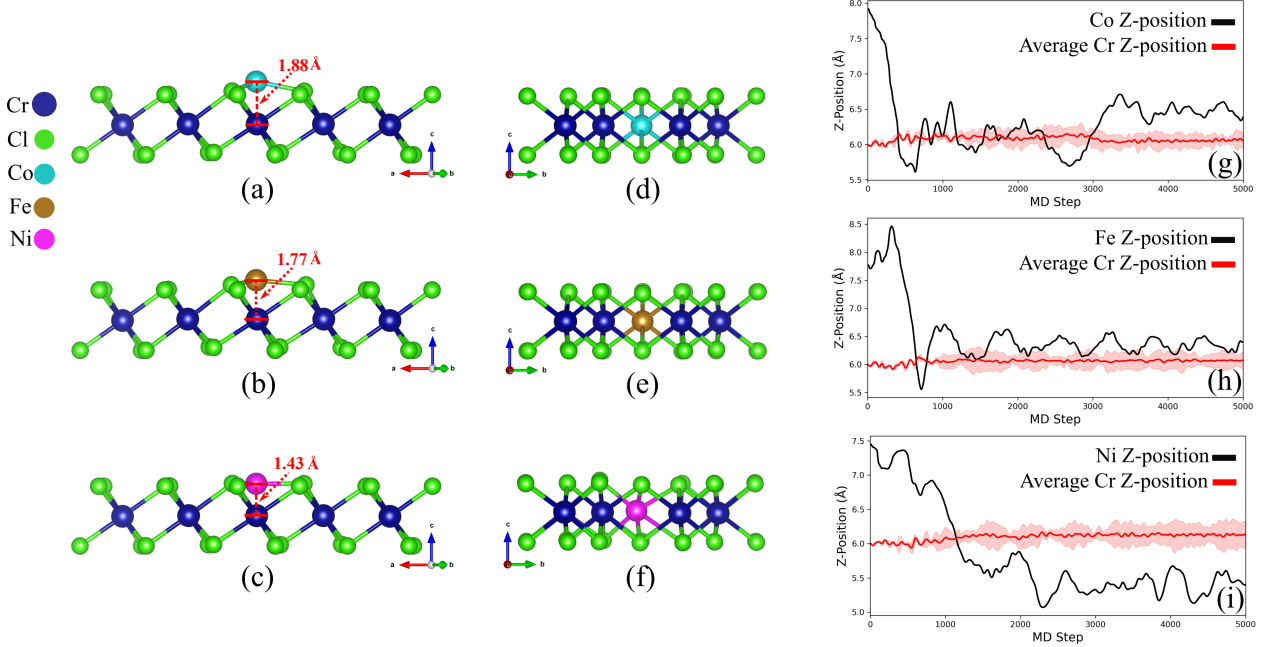
Figure 3: Structural configurations and finite-temperature evolution of Co-, Fe-, and Ni-functionalized monolayer CrCl 3 . (a–c) Optimized surface-adsorbed configurations at the threefold surface hollow site ( S_2 ) considering U_{Cr} = 3.29 eV and vdW corrections. (d–f) Corresponding embedded configurations ( \Delta z_{Cr-TM} \approx 0.0 Å). (g–i) Absolute TM z coordinates during 5 ps AIMD simulations at 300 K. Black curves denote the transition-metal positions; red curves and shaded regions represent the average Cr-plane position and its fluctuations.
