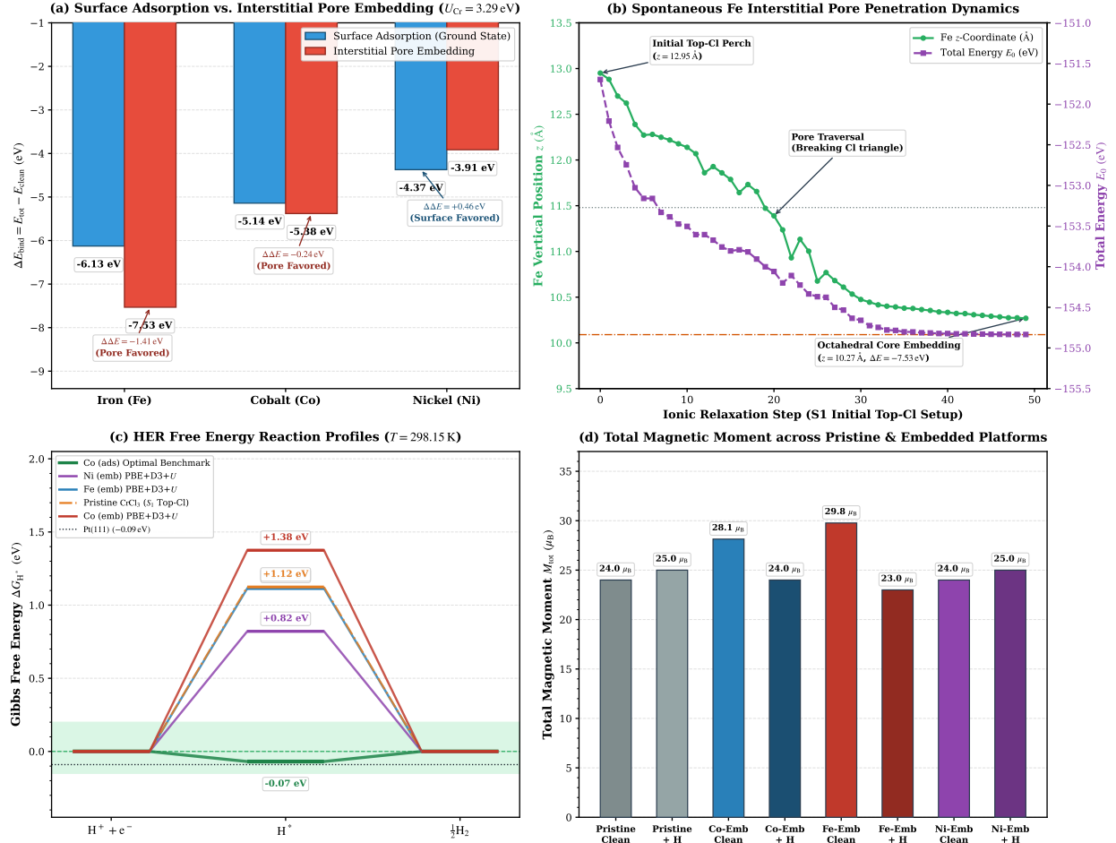
Figure S7. Structural stability, spontaneous dynamics, and electrocatalytic response of interstitial single-atom transition-metal (TM = Fe, Co, Ni) embedded monolayer CrCl 3 . (a) Comparison of surface adsorption (hollow site) versus interstitial pore embedding binding energies ( \Delta E_{bind} = E_{tot} - E_{clean} - E_{TM} ) under PBE+D3+U ( U_{Cr} = 3.29 eV). Fe ( \Delta\Delta E = -1.41 eV) and Co ( \Delta\Delta E = -0.24 eV) thermodynamically favor interstitial pore incorporation, whereas Ni ( \Delta\Delta E = +0.46 eV) prefers surface adsorption. (b) Spontaneous vertical penetration dynamics of Fe initially placed at the S_1 (top-Cl) perch during geometry relaxation, illustrating barrierless sinking into the octahedral interstitial core ( z \approx 10.27 Å) and global energy minimization. (c) Free energy reaction profiles for HER atop embedded TM centers compared to pristine top-Cl and surface-adsorbed Co, highlighting that octahedral coordination shields TM-3d active centers and leads to high free energy barriers ( \Delta G_{H^*} \geq +0.82 eV). (d) Total magnetic moment ( M_{tot} ) across pristine and embedded configurations before and after hydrogen adsorption, illustrating local spin compensation upon H coordination.
