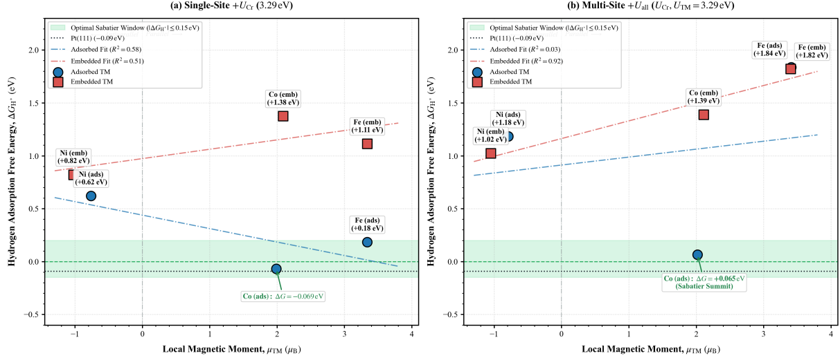
Fig. S5. Relationship between the local magnetic moment of the functionalizing transition-metal atom, \mu_{\text{TM}} , in the relaxed H-free configurations and the hydrogen adsorption free energy, \Delta G_{\text{H}^*} , across two systematic Hubbard U tiers: (a) single-site +U_{\text{Cr}} ( U_{\text{Cr}} = 3.29 eV) and (b) multi-site +U_{\text{all}} ( U_{\text{Cr}} = U_{\text{TM}} = 3.29 eV). Blue circles and red squares represent the surface-adsorbed ( S_2 ) and embedded transition-metal configurations in monolayer \text{CrCl}_3 , respectively. The vertical dash-dotted line at \mu_{\text{TM}} = 0 separates antiparallel (Ni) from parallel (Co, Fe) magnetic coupling relative to the ferromagnetic Cr host. Shaded green bands denote the optimal Sabatier catalytic window ( |\Delta G_{\text{H}^*}| \leq 0.15 eV) with the Pt(111) benchmark ( -0.09 eV) indicated by dotted horizontal lines. Magnetic moments are expressed in units of the Bohr magneton, \mu_B .
