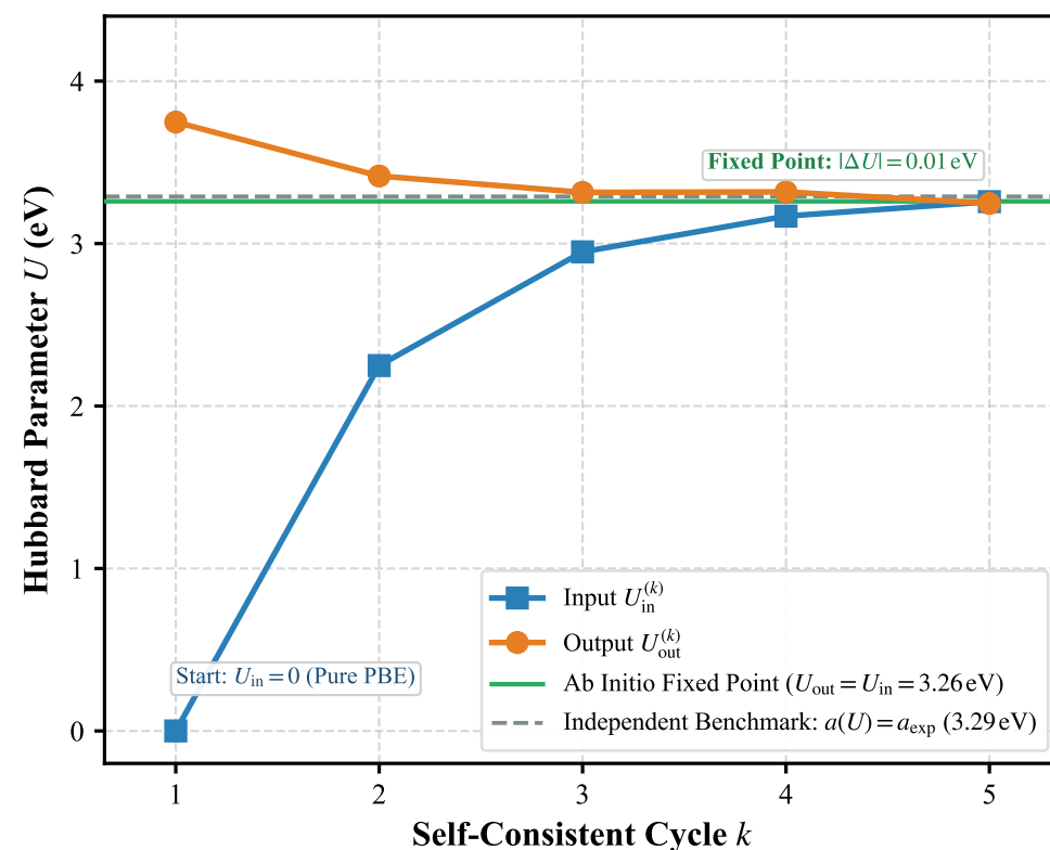
(b) Kulik–Marzari Self-Consistent Feedback Convergence
