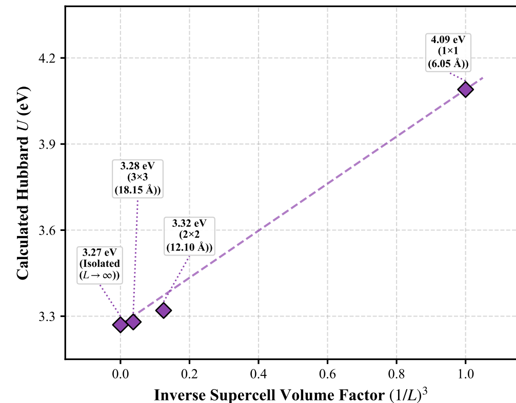
(c) Supercell Finite-Size Scaling & Periodic Image Screening
