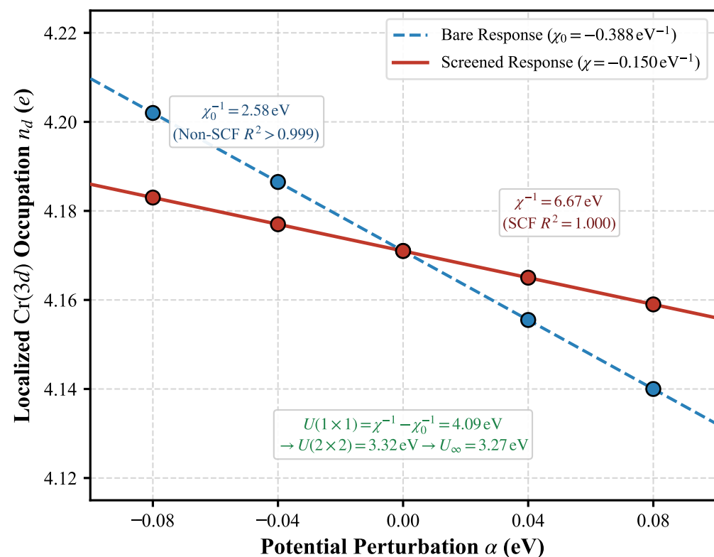
(a) Ab Initio Cococcioni Linear Response on Monolayer \text{CrCl}_3
