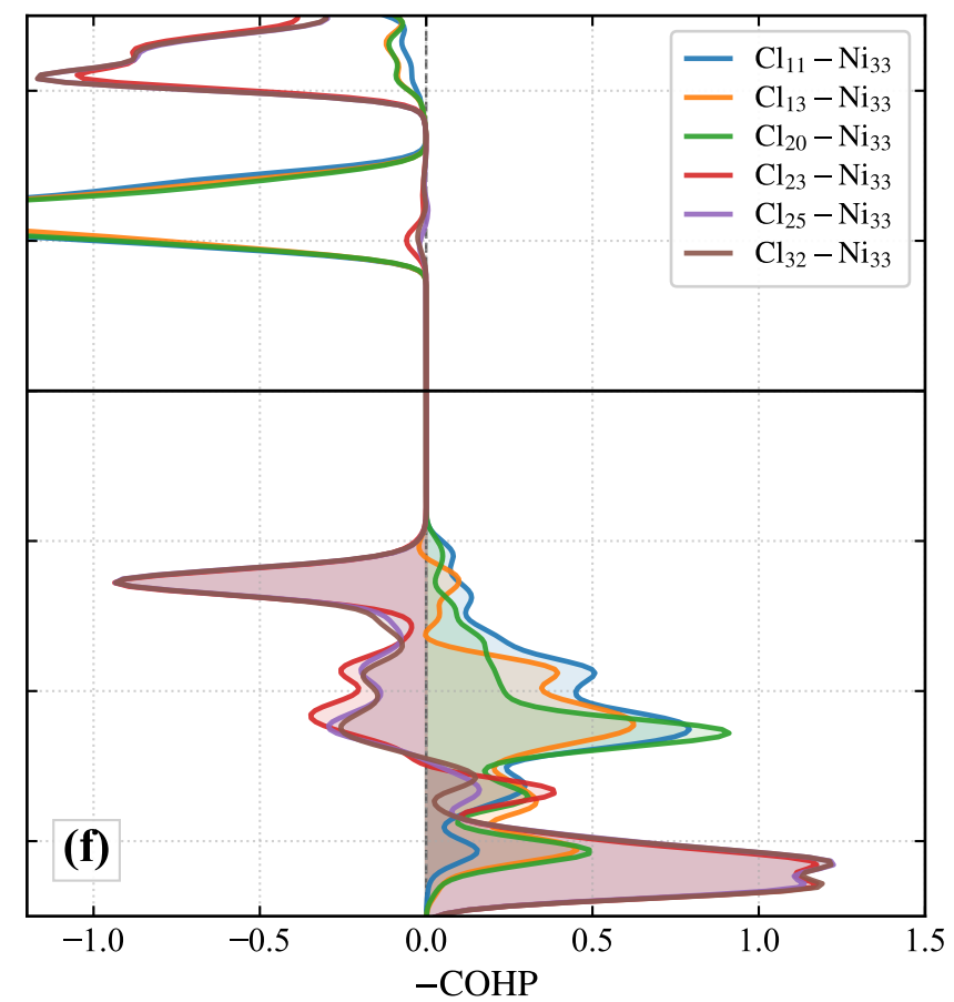
CrCl 3 --Ni (embedded)
