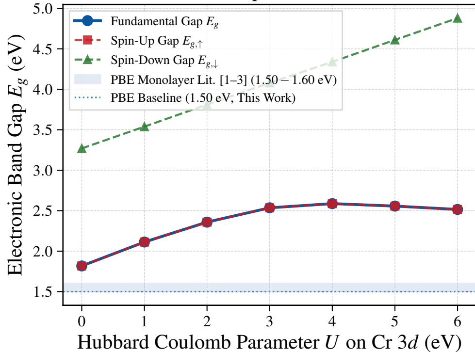
(a) Band Gap vs. Hubbard U
