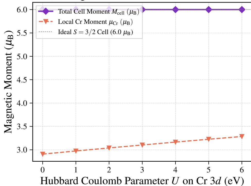
(b) Magnetic Ground State vs. Hubbard U
