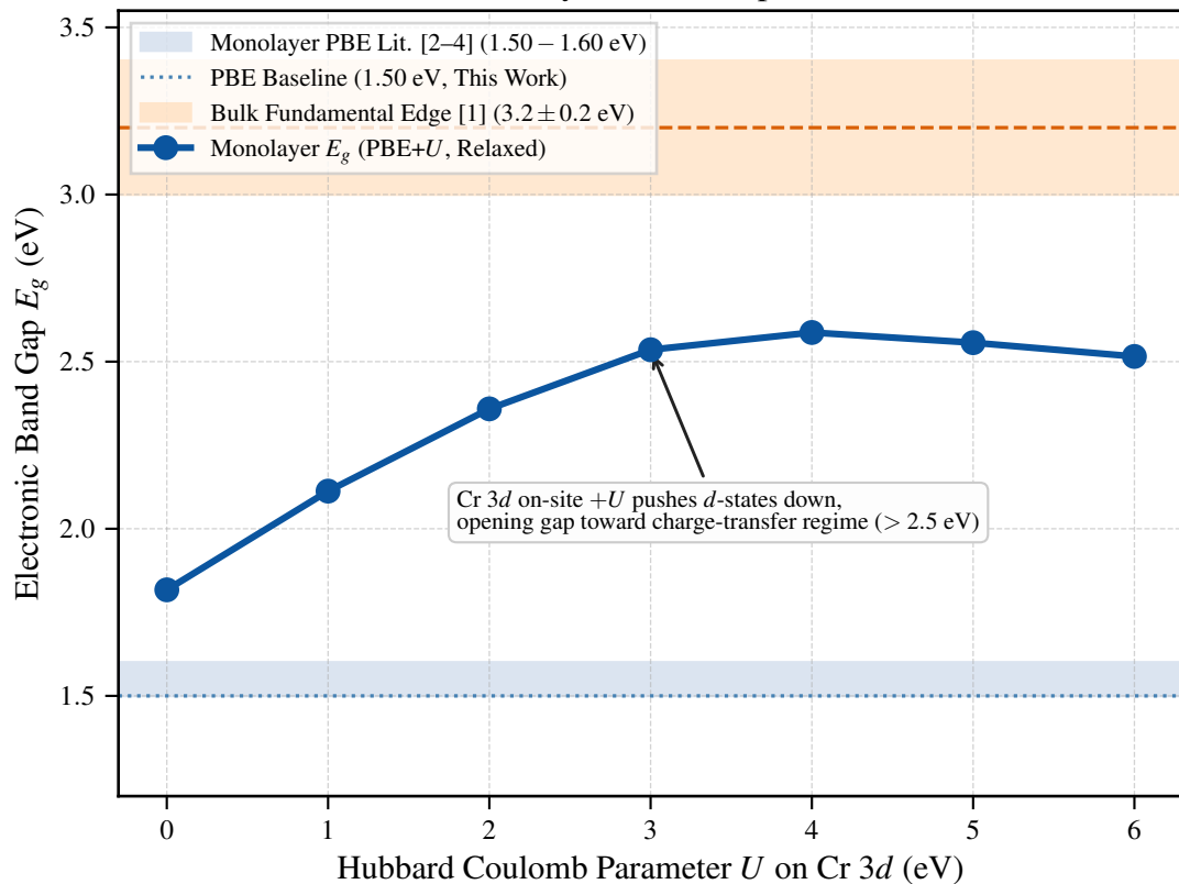
(a) CrCl 3 Monolayer: Band Gap vs. Hubbard U
