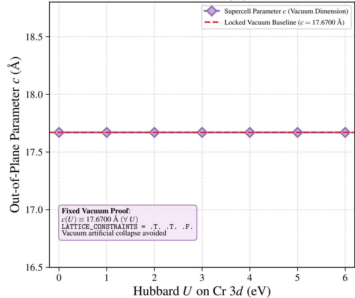
(c) Out-of-Plane Parameter c(U) (Vacuum Fixed)
