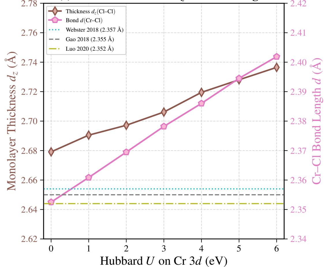
(e) Vertical Thickness d_z & Bond Length
